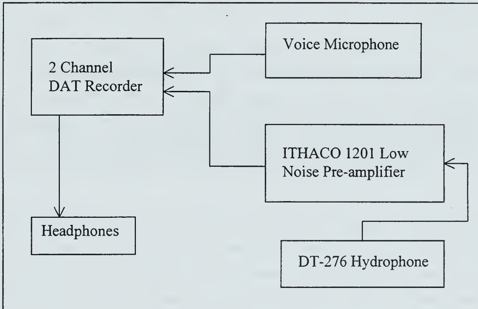
Figure 3.1. Recording equipment setup.
